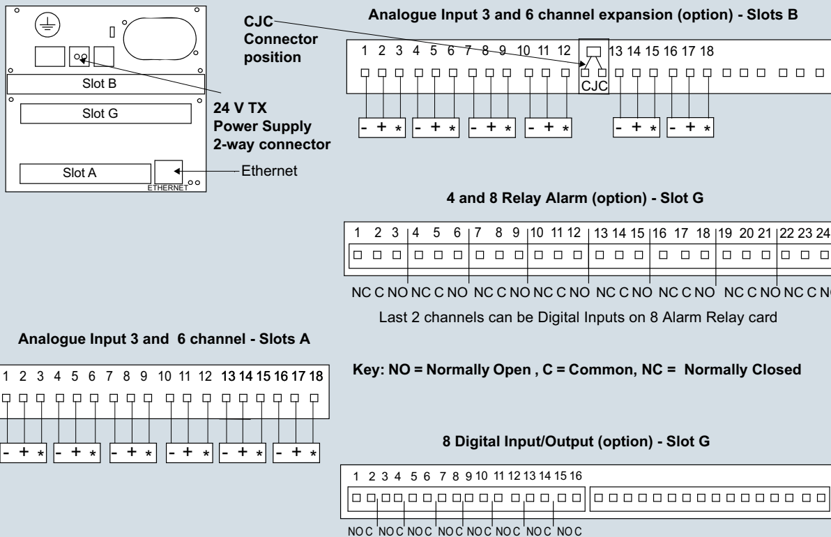
SIREC D200 - Terminal assignments and power requirements (rear of unit)
